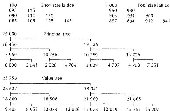
FIGURE 14.14 Quick's CMO valuation. The top of the figure shows the short rate lattice. Next to that is the lattice showing the corresponding pool size fraction. These lattices start at the top and move downward. A down move is a move directly downward, and an up move is a move downward to the right. Below these is the tree of principal due class A, and finally the corresponding tree of values for class A.
