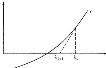
FIGURE 2.4 Newton's method
