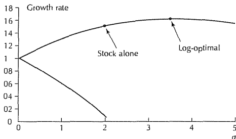
FIGURE 15.6 Feasible region for one stock and a risk-free asset. The log-optimal strategy gives only modest improvement in growth rate over holding the stock alone, at the expense of a greatly increased standard deviation.
