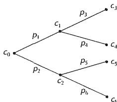
FIGURE 16.11 Two-period project. The buying price can be found by evaluating the certainty equivalent by a backward process
