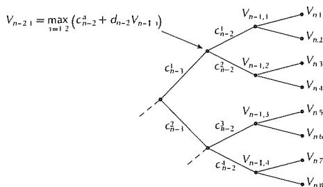
FIGURE 5.7 Second stage of dynamic programming. Assuming that the first n-2 stages of the process have been completed, we evaluate the best running present value for the remaining two stages.
