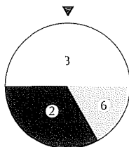
FIGURE 6.5 Betting wheel. It is possible to bet on any segment of the wheel. If that segment is chosen by the spin, the bettor receives the amount indicated times the bet.
