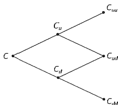
FIGURE 12.6 Two-period option The value is found by working backward a step at a time.
