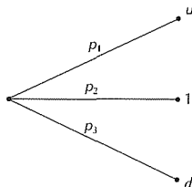
FIGURE 13.6 One piece of a trinomial lattice. In this lattice we must have d = 1/u so that the nodes recombine after two steps
