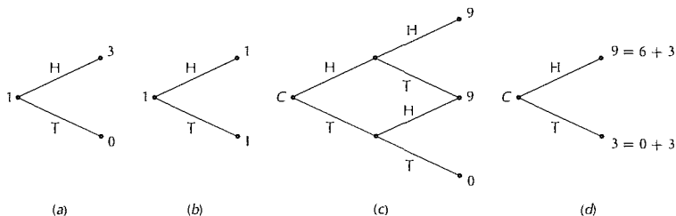
FIGURE 12.14 A proposition and its parts Tree (a) is a basic risky proposition; tree (b) is a risk-free opportunity; and tree (c) represents a new, more complex proposition. The value C can be found by breaking it into its parts. The final piece is shown in (d).
