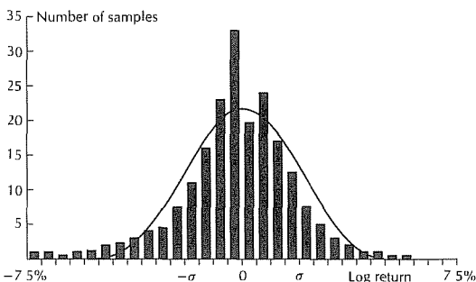
FIGURE 11.3 Observed distribution of the logarithm of return. The distribution has “fatter tails” than a normal distribution of the same variance
