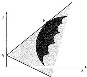
FIGURE 6.14 One-fund theorem When both borrowing and lending at the risk-free rate are allowed, there is a unique fund F of risky assets that is efficient. All points on the efficient frontier are combinations of F and the risk-free asset.
