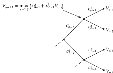
FIGURE 5.6 First recursive step of dynamic programming. Assuming that the first n-1 steps of the process have been completed, we evaluate the best that can be done for the last step. For any node at time n-1 we find the maximum running present value from that node.
