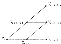
FIGURE 14.3 No arbitrage is possible. The initial price P_{ti} is determined by discounted risk-neutral valuation. If all payoffs are nonnegative, then the initial price must also be nonnegative.
