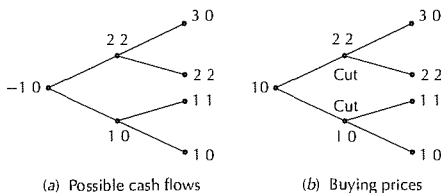
FIGURE 16.12 Buying price for tree farm. (a) Cash flow generated at a node if the trees are cut at that point. (b) Certainty equivalent at a node and best policy
