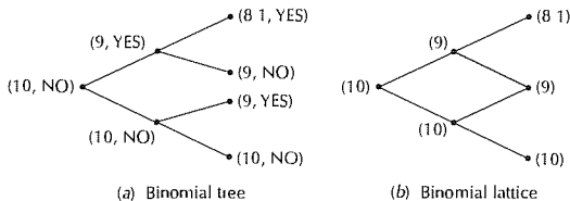
FIGURE 5.4 Trees showing oil well states. Pumping corresponds to an upward movement; no pumping corresponds to a downward movement. The tree in (a) accounts for both the level of reserves and the status of a crew. If only the reserve levels affect the profit, some nodes combine, forming a binomial lattice, as shown in (b).
