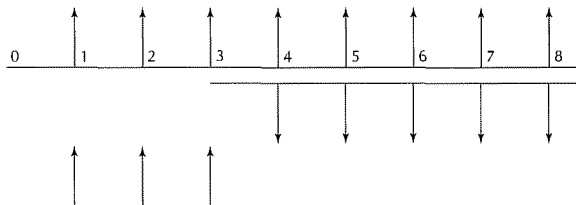
FIGURE 3.2 Finite stream from two perpetual annuities. The top line shows a perpetuity starting at time 1, the second a negative perpetuity starting at time 4. The sum of these two is a finite-life annuity with payments starting at time 1 and ending at time 3.
